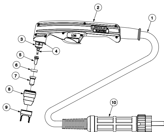
LC65 Optional Nozzles & Related Accessories
