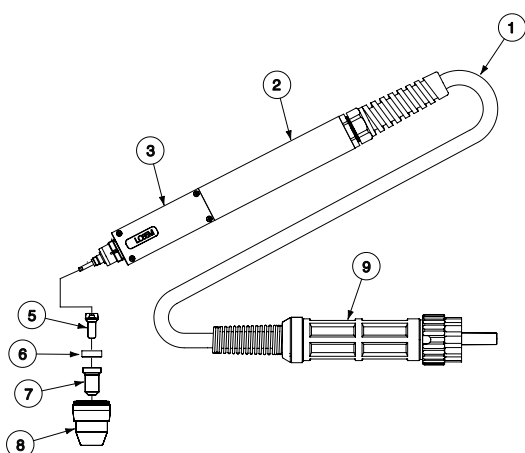
LC65M Optional Nozzles & Related Accessories
